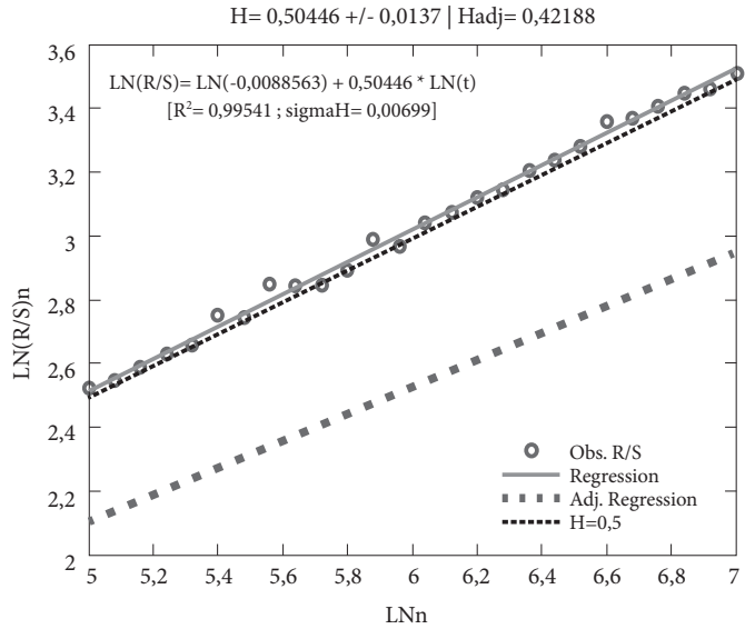
Figure 4. Walmart and JP Morgan (adjusted and unadjusted Hurst exponent)
