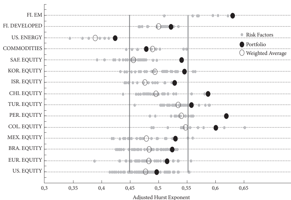
Figure 5. Adjusted Estimated Hurst Exponent ( \square ) 7
