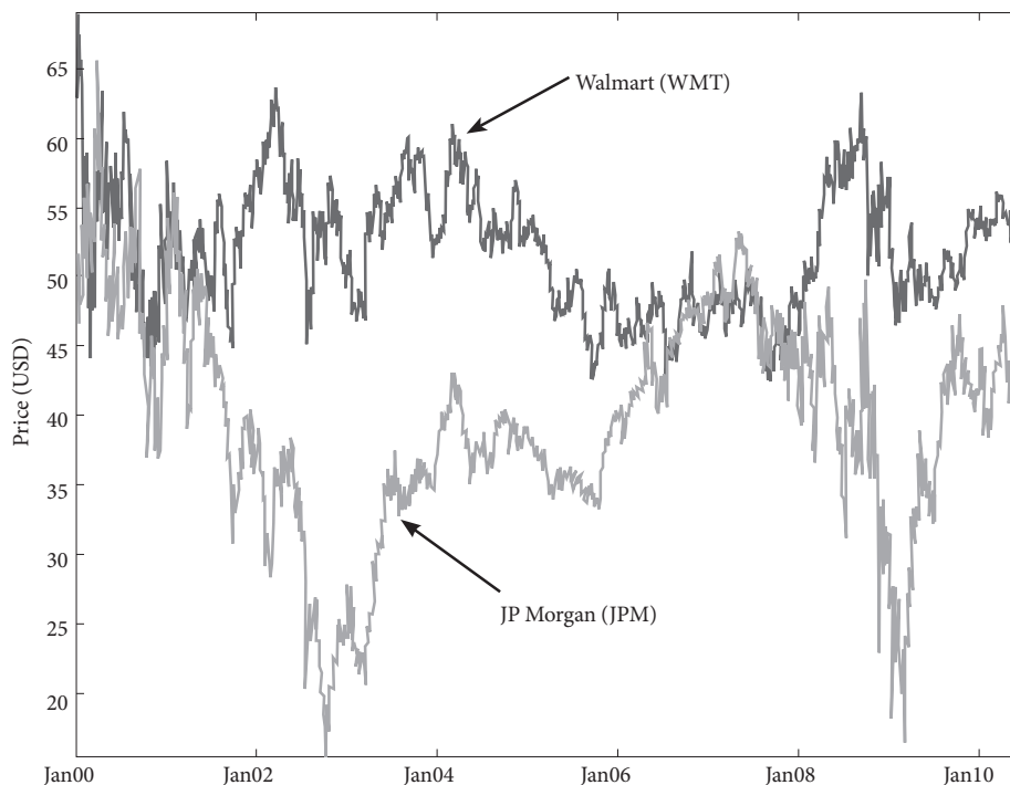
Figure 3. Daily prices for Walmart and JP Morgan
