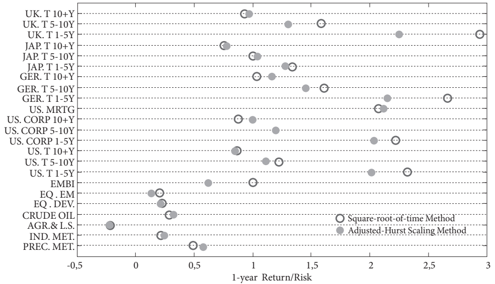
Figure 6. Return/Risk Ratio for the Standard and the Enhanced Methods
