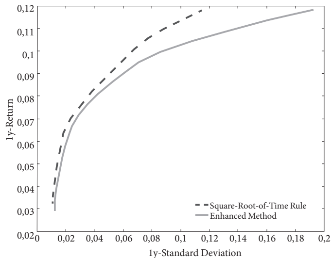
Figure 1. Efficient Frontiers for the Standard and the Enhanced Methods 1-year
