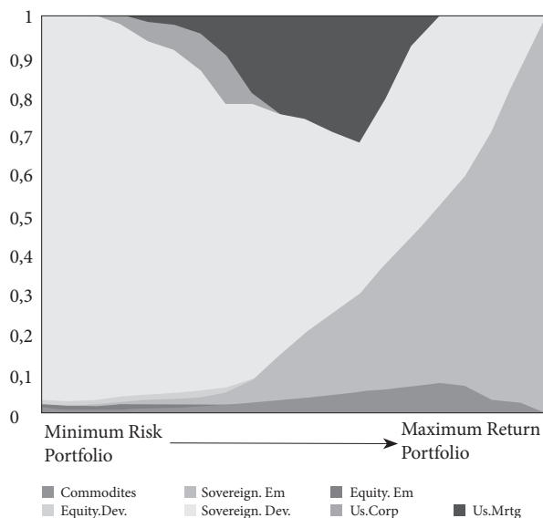
Figure 8. Square-Root-of-Time and Adjusted-Hurst Methods for 1 year and 10 year Weights H=0.5 ( n -year)
