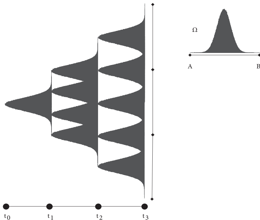
Figure 2. Independence and the Square-Root-of-Time Rule Independent Process
